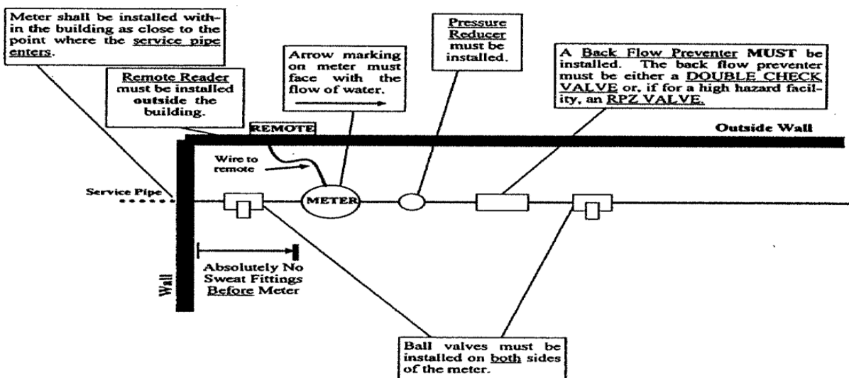
Diagram for Water Meter/Remote Installation
